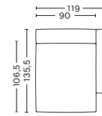
Right armrest Art. S8261 W90/119 x D106,5/135,5 x H37/67 cm Armrest D29 cm
